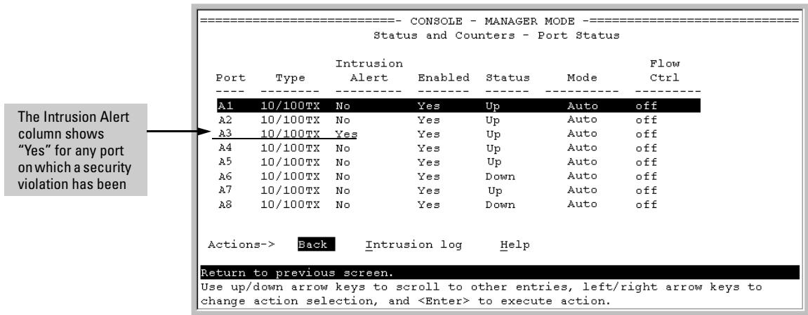
Figure 13-13. Example of Port Status Screen with Intrusion Alert on Port A3
